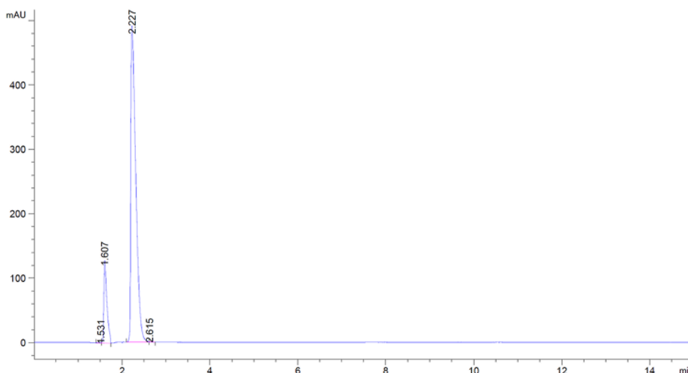
HLPC trace:
